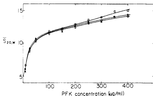
FIGURE 5: \bar{s}_{20,w} as a function of PFK concentration for the PFK preparations in TEMA buffer at pH 7.0, 23 °C. The symbols and preparations of PFK are as described in Figure 1. The lines represent the theoretical fit of the experimental data using the association model of M_1 \rightleftharpoons M_4 \rightleftharpoons M_{16} and other parameters shown in Table IV. The data points are the average of multiple data sets.
